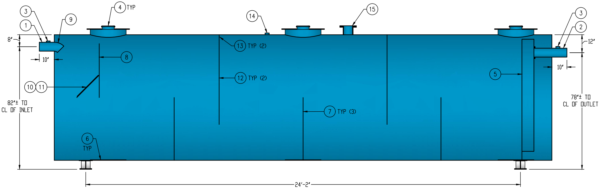
SECTION VIEW
