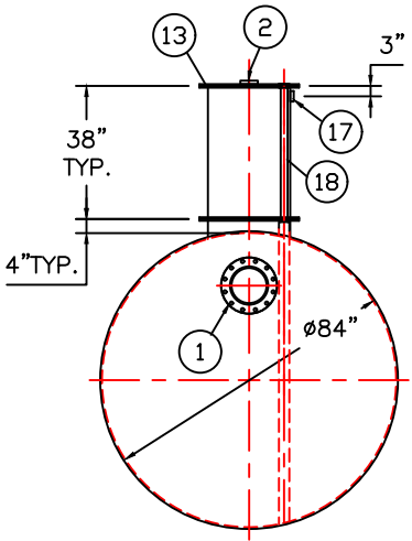
END VIEW
