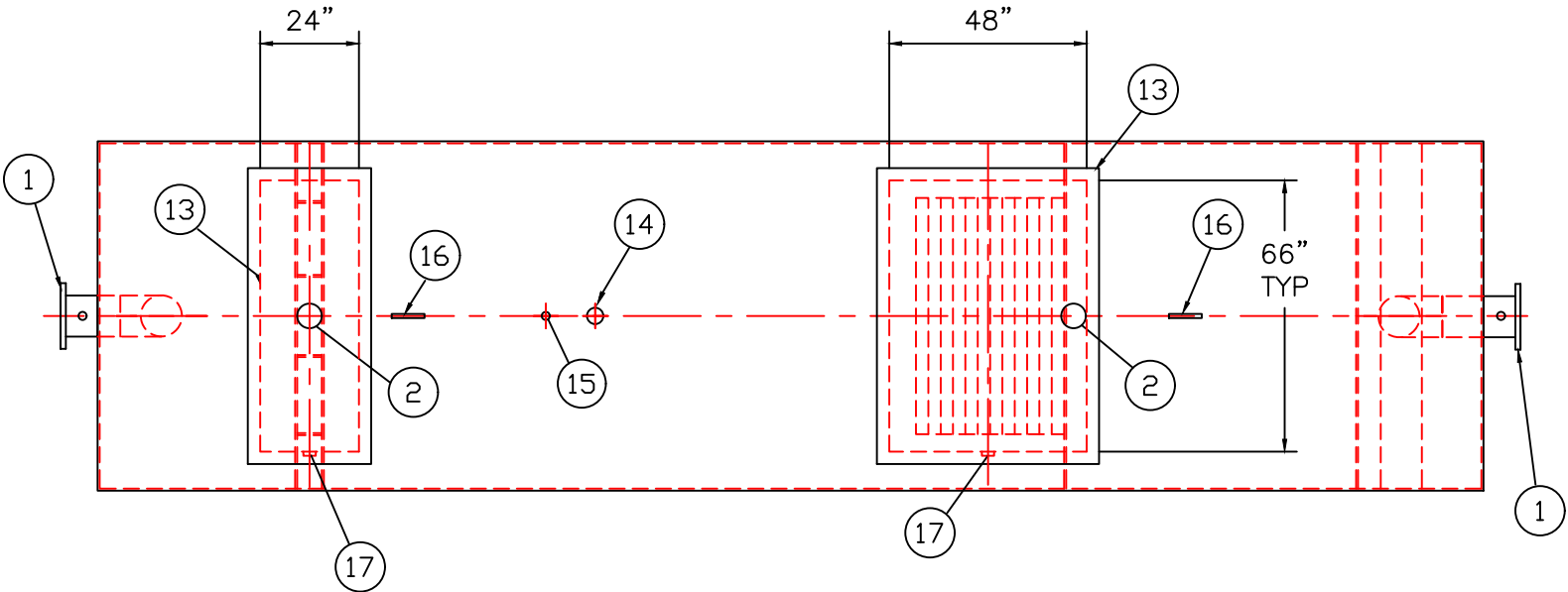
PLAN
