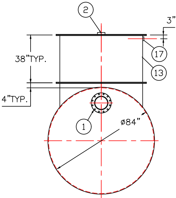
END VIEW
