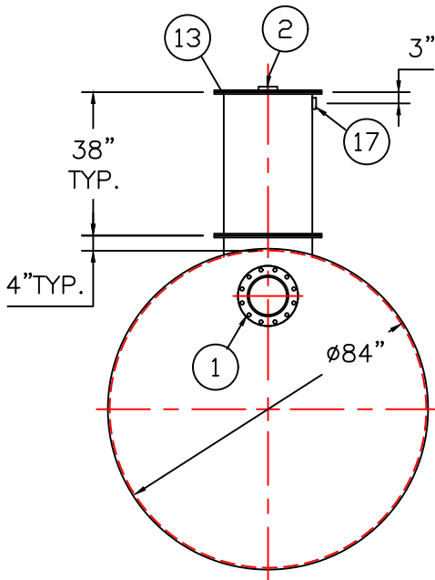
END VIEW
