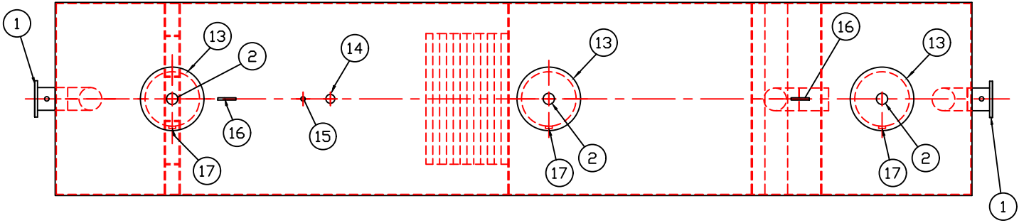
PLAN
