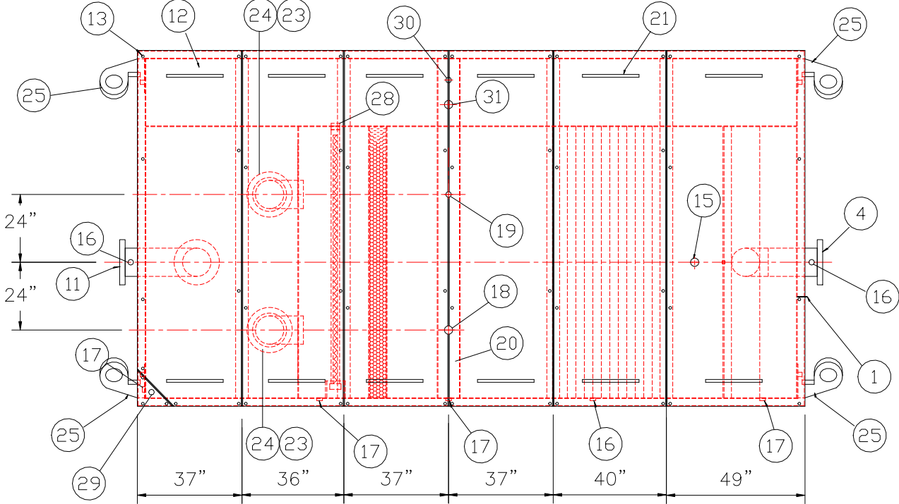
REMOVABLE COVERS (6) REQUIRED PLAN VIEW
