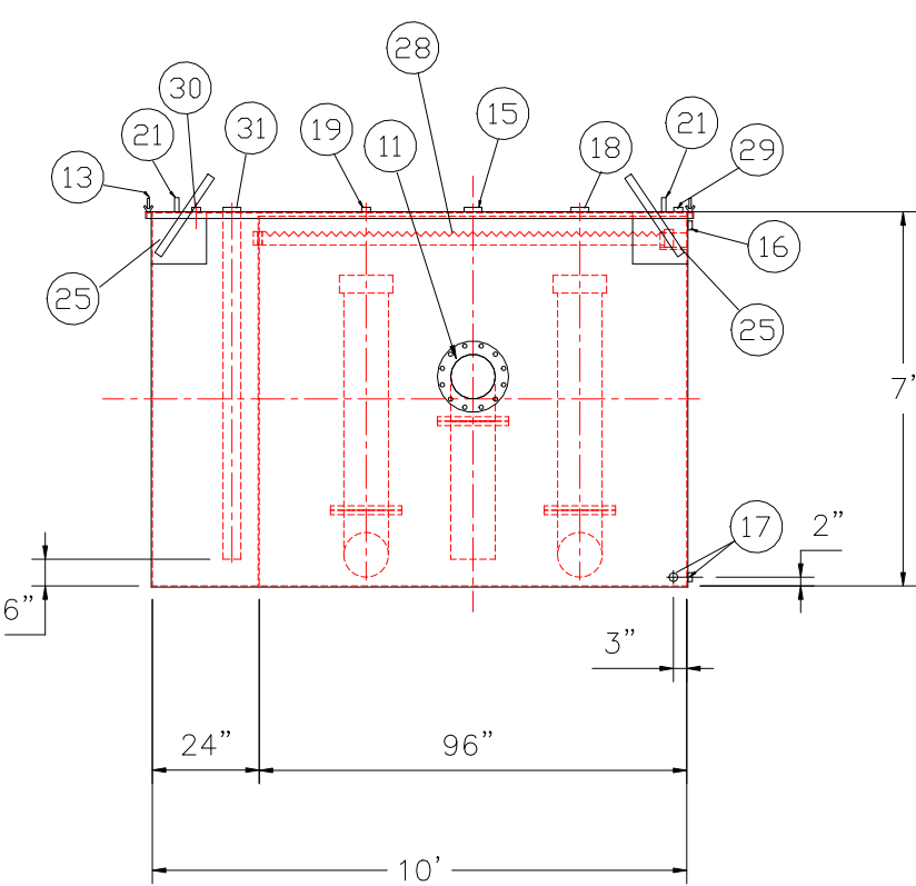
END VIEW
