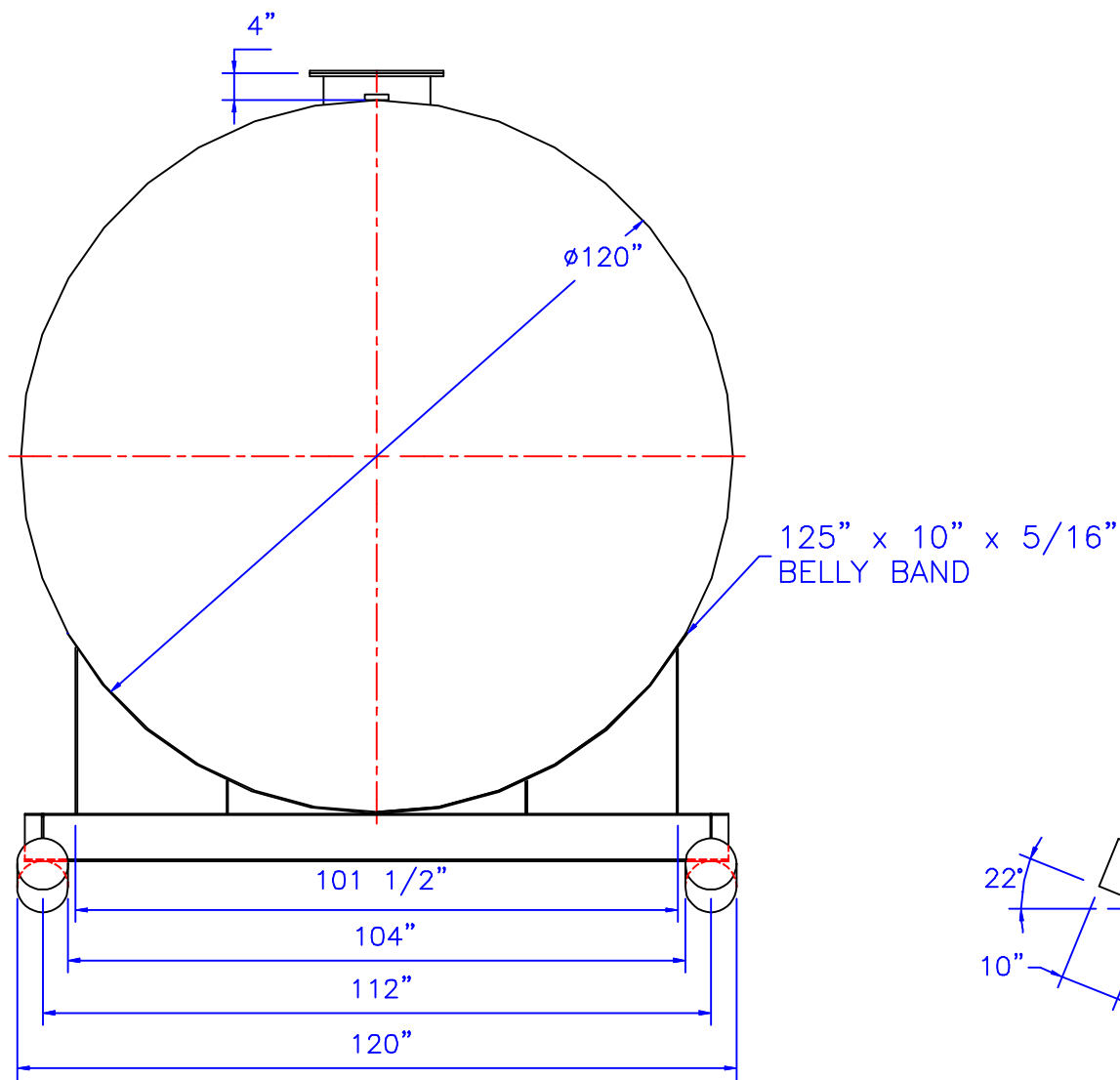
END VIEW
