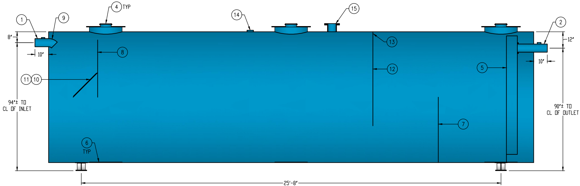
SECTION VIEW
