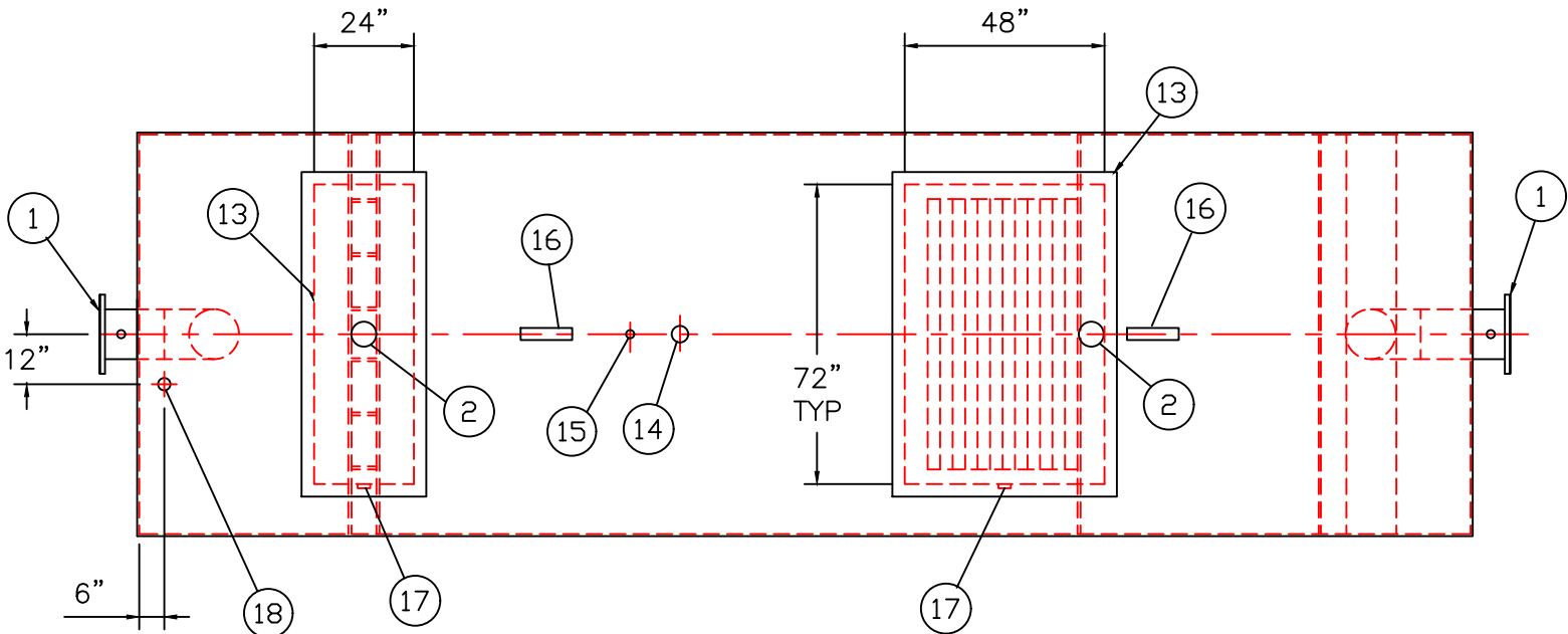
PLAN VIEW
