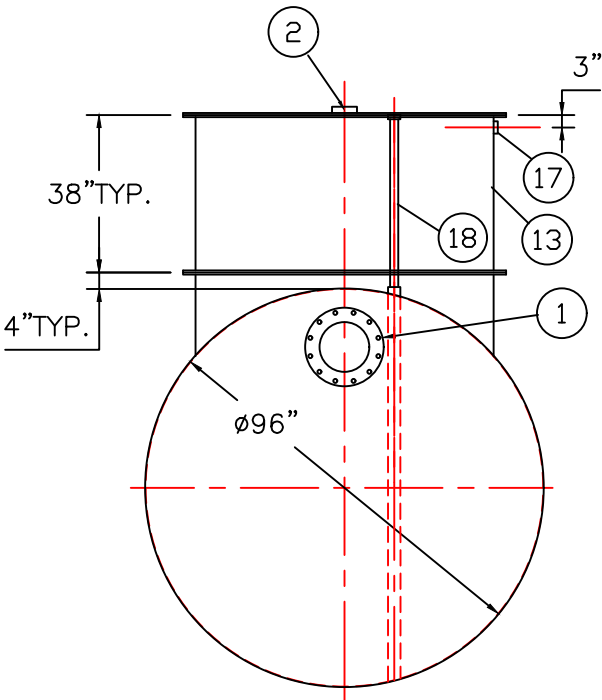
END VIEW
