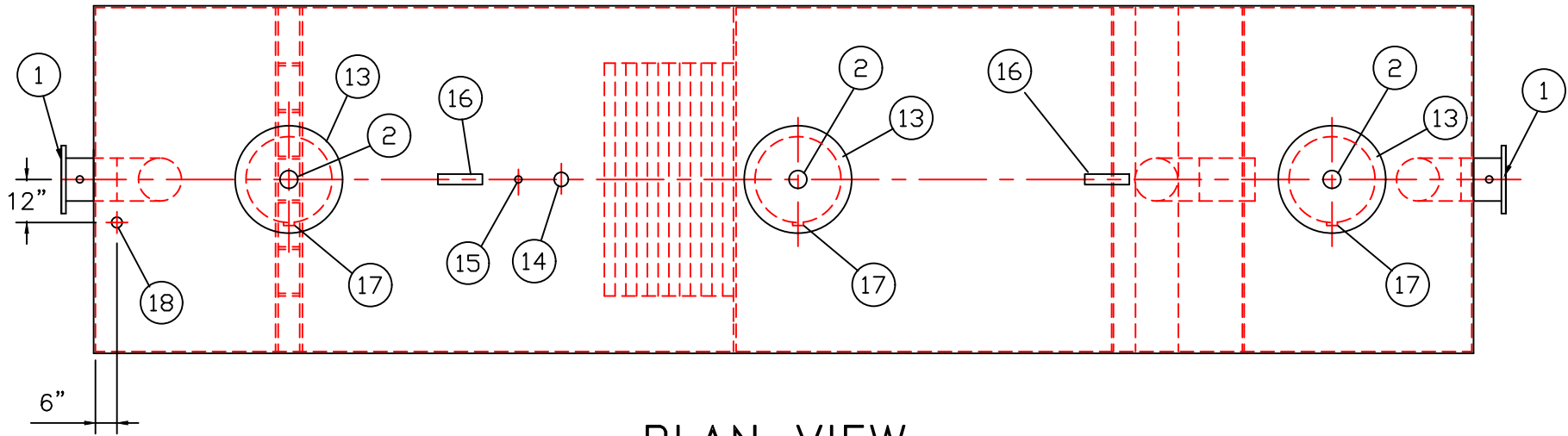
PLAN VIEW
