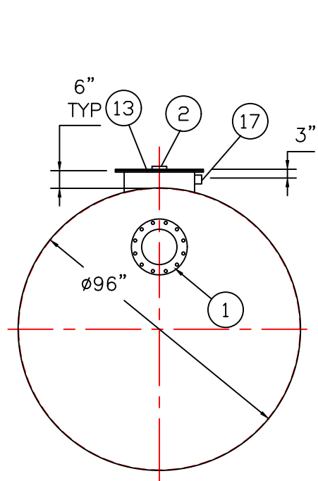
END VIEW
