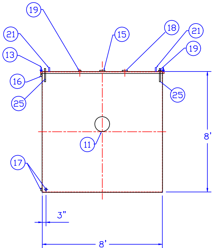
END VIEW
