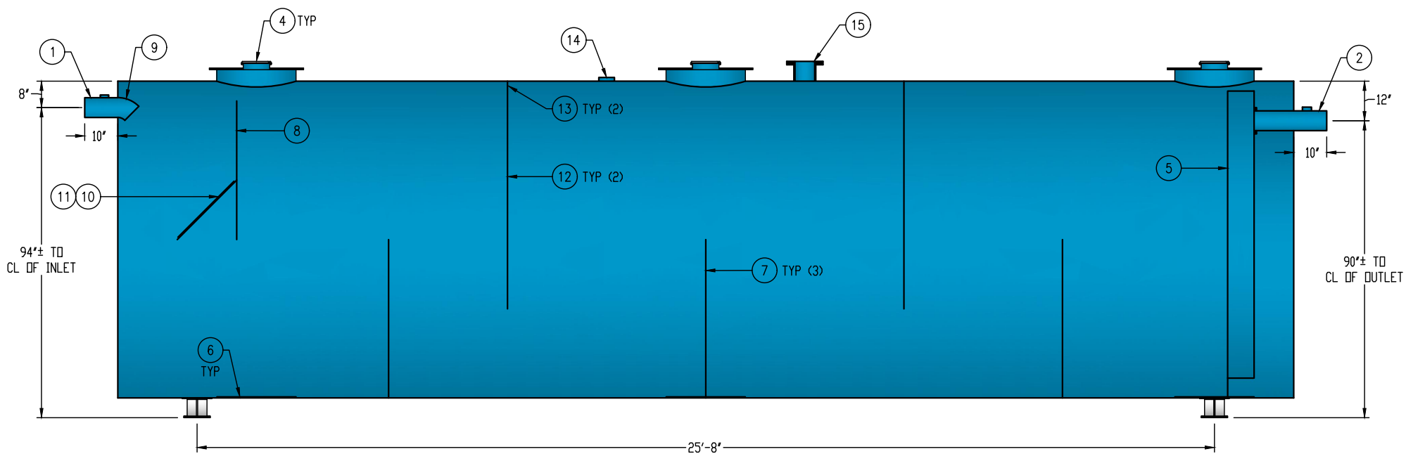
SECTION VIEW
