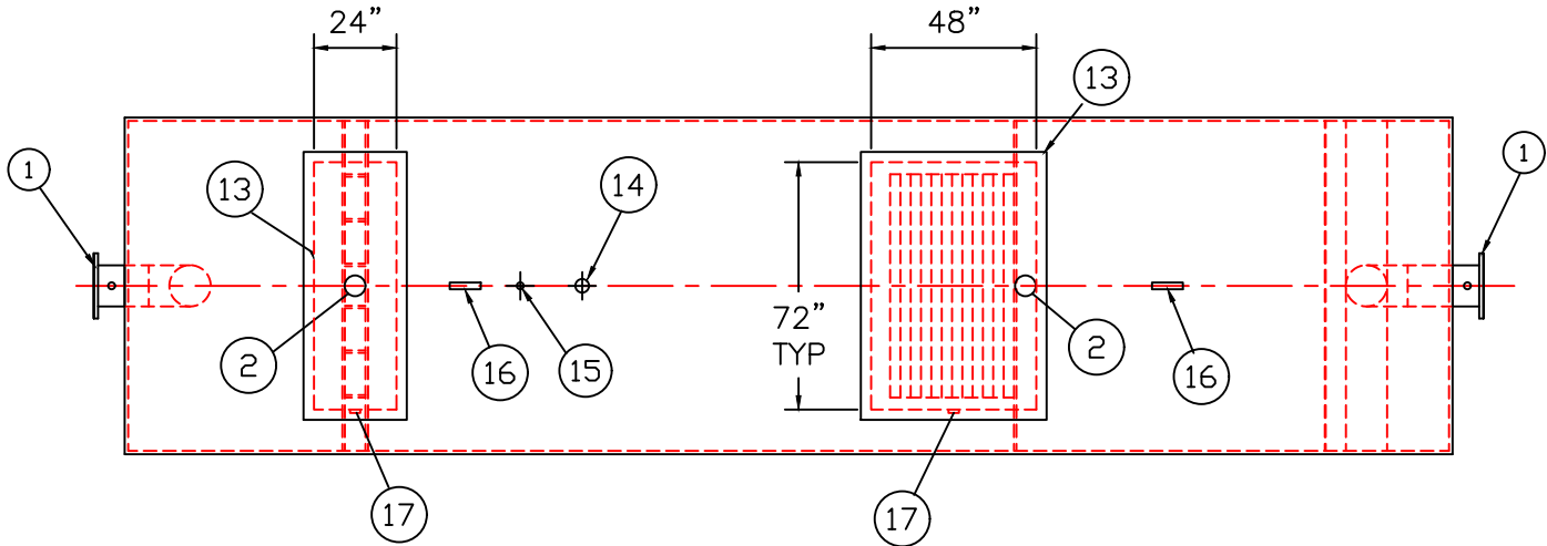
PLAN VIEW
