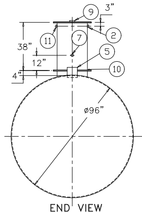
END VIEW
