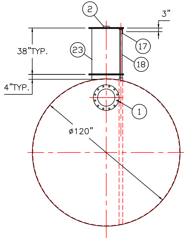
END VIEW
