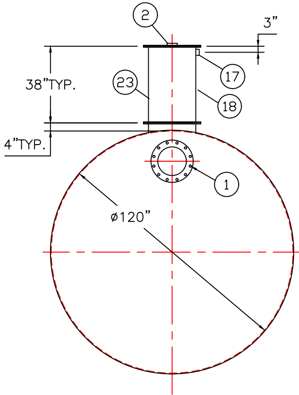
END VIEW
