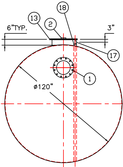
END VIEW
