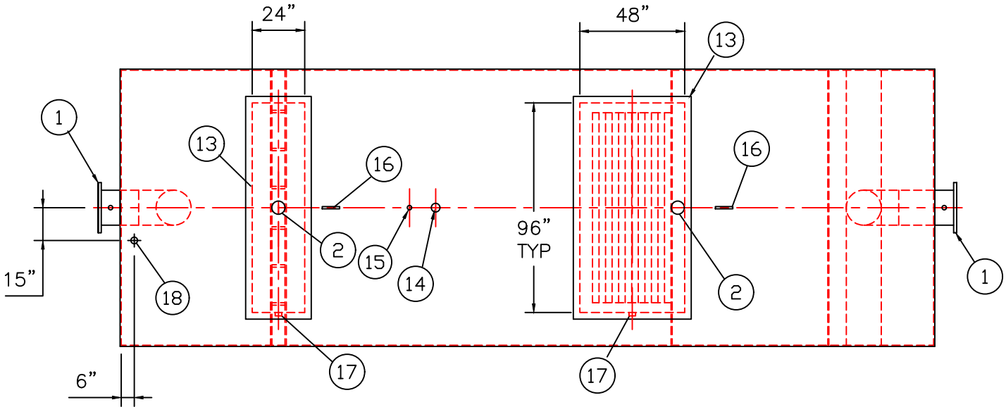
PLAN
