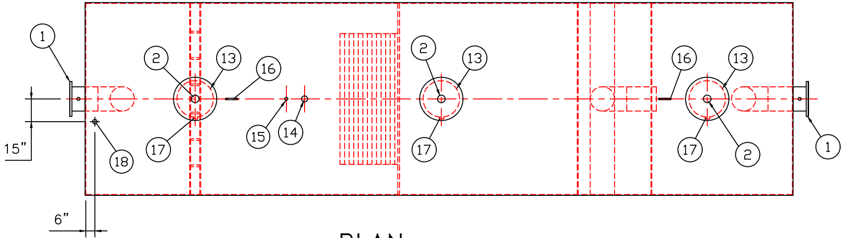
PLAN
