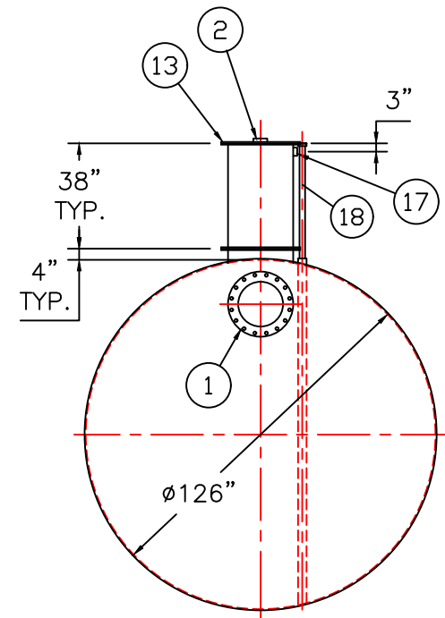
END VIEW
