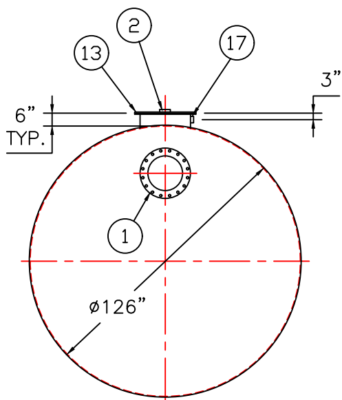
END VIEW
