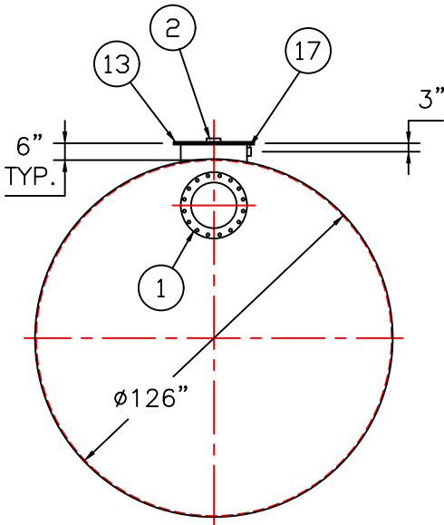
END VIEW
