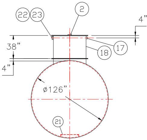
END VIEW
