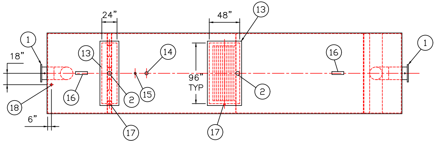
PLAN
