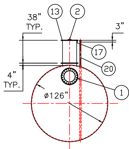
END VIEW
