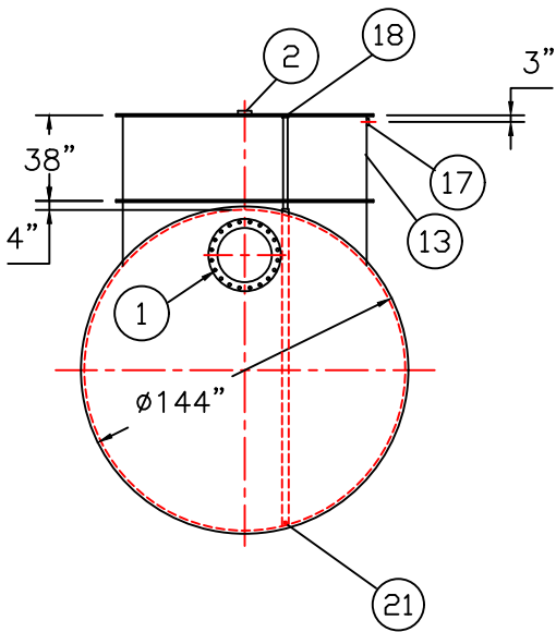
END VIEW
