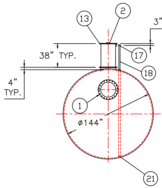
END VIEW
