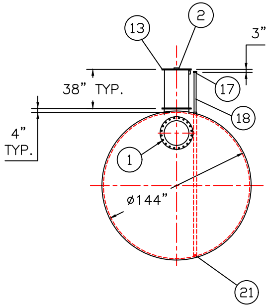
END VIEW
