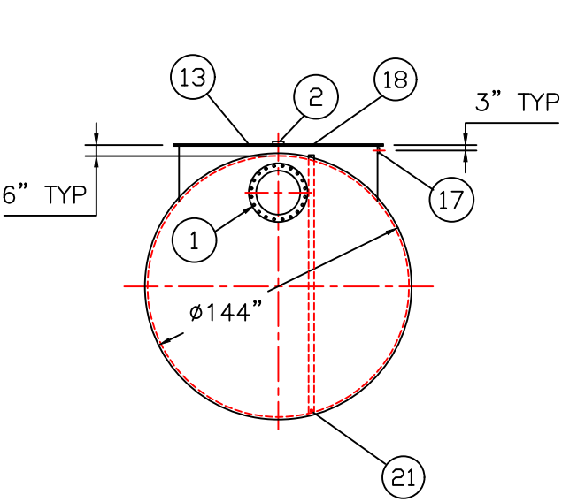
END VIEW
