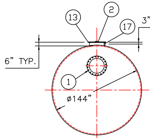
END VIEW
