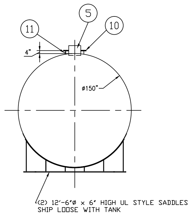
END VIEW
