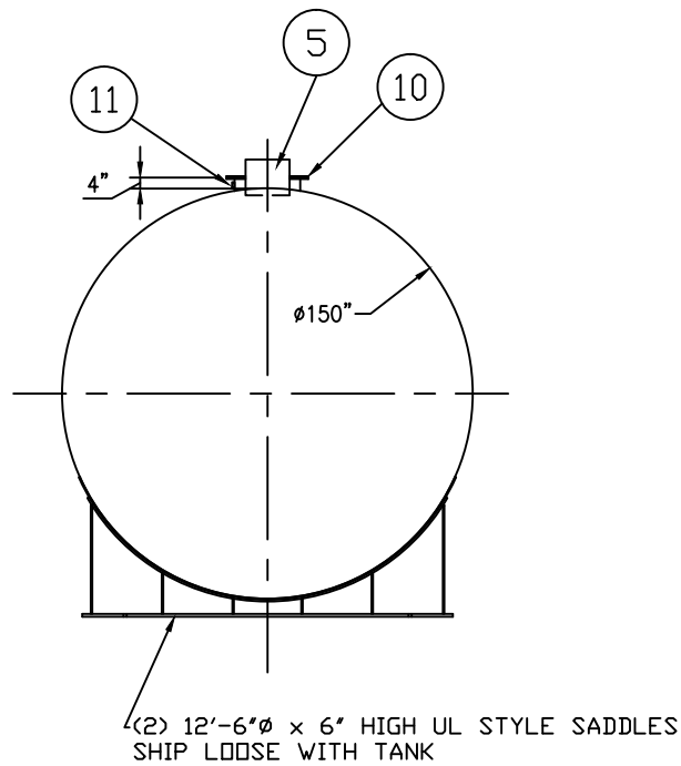
END VIEW
