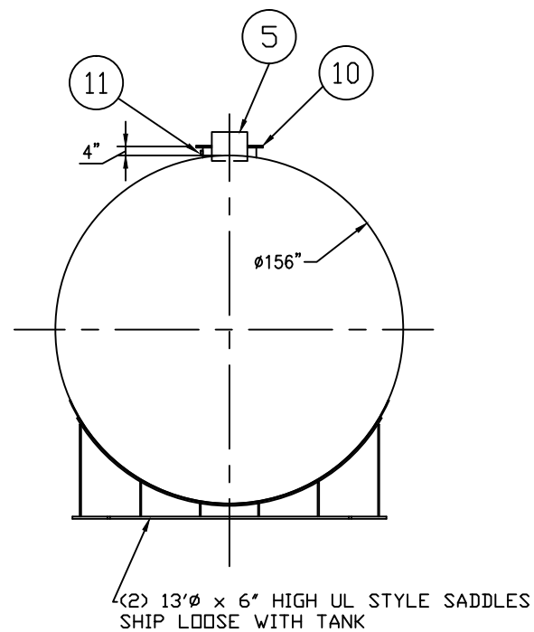
END VIEW
