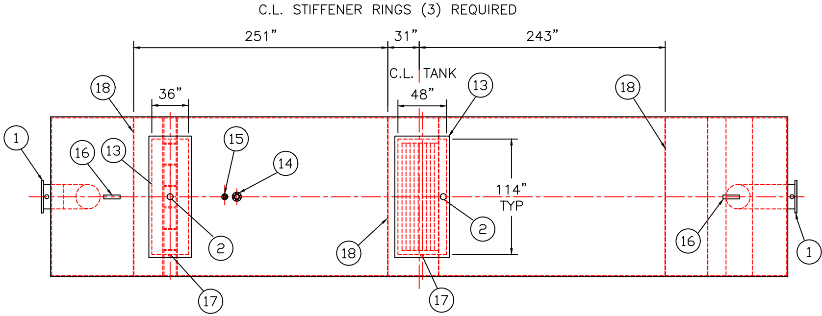
PLAN
