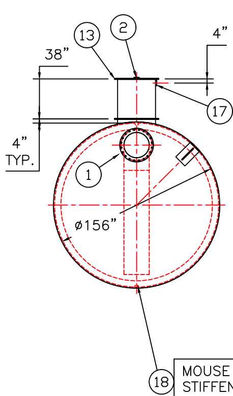
END VIEW
