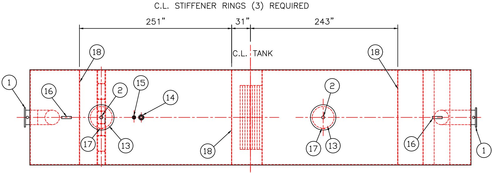
PLAN
