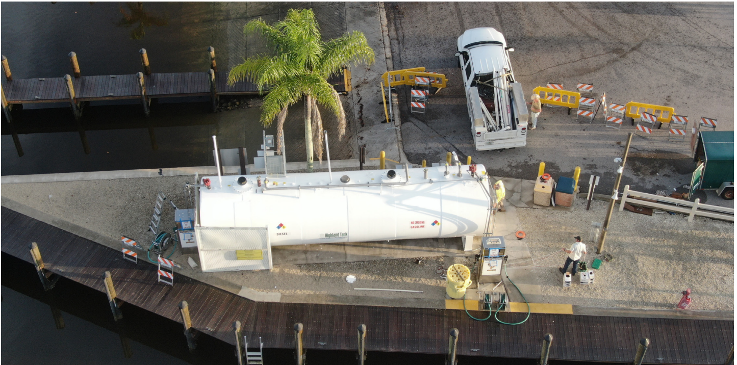
Compartmented Fireguard Tank for marina fueling.
