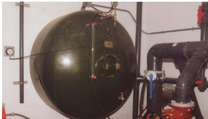
30,000 gallon ASME Fire Protection Tank
